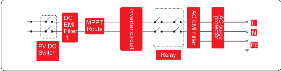
Figure 2.8 Diagramma circuitale
