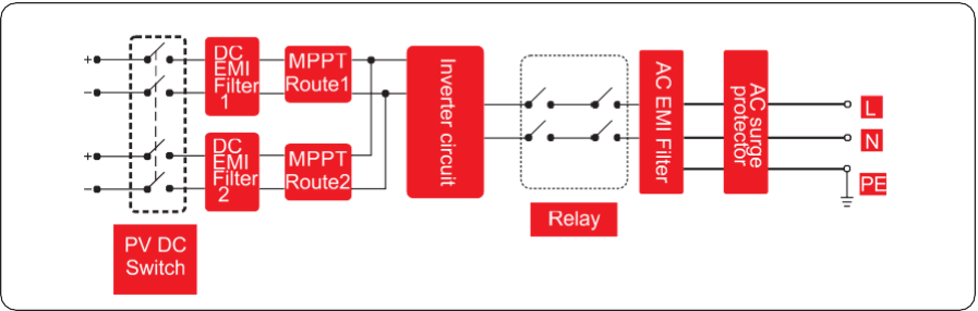
Figure 2.9 Diagramma Circuitale
