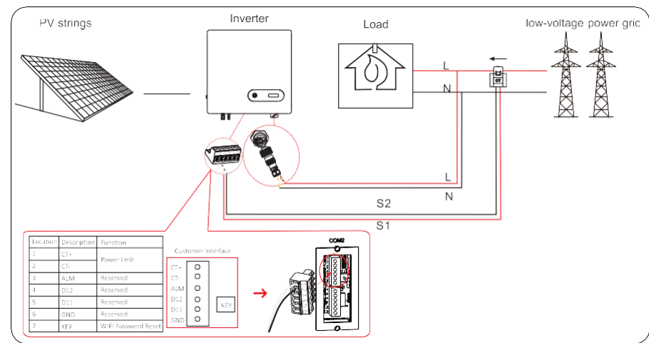
Figure 5.16 Diagramma cablaggio Inverter+CT
