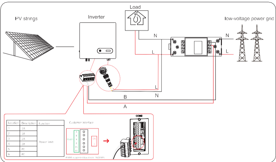
Figure 5.18 Diagramma cablaggio Inverter+Meter
